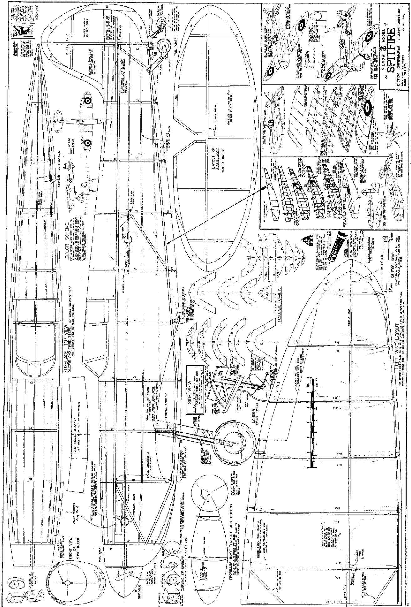
This great Golden Era plan was donated by Sam Brewer, of Phoenix, Arizona. Check your local hobby shop for a molded canopy you could modify to improve the appearance. Note shortened location of rear motor hook; it eliminates tail-heavy problem because of heavy rubber motor.
