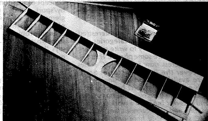
Wing center section before adding pine block for hold-down bolt. Single nylon bolt holds wing in place.
