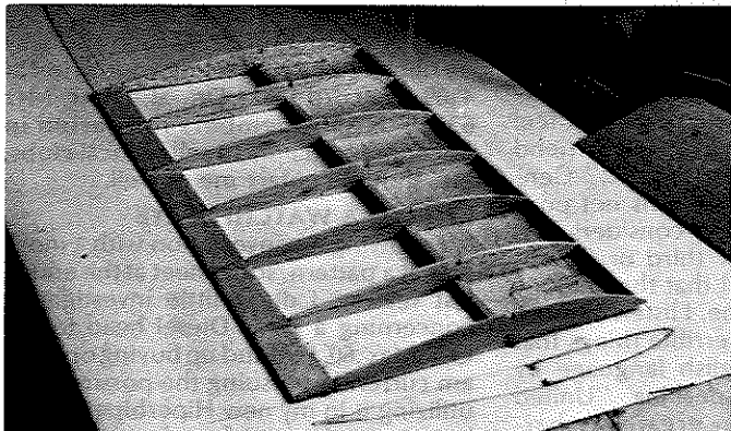
Wing is basically built from 1/16 sheet, sanded to 1/20. Careful wood selection is important to avoid excess weight.
