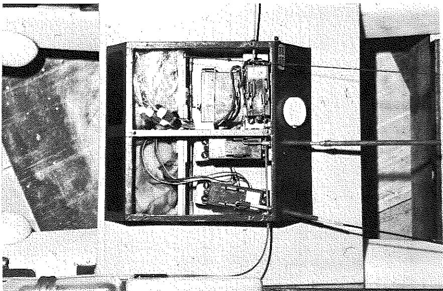
R/C equipment installation in Sealand II. Cover is gasketed to keep out water. Servos, linkages, and other gear easily accessible. Pill bottle top idea by Lenny Poor. Really works well.
