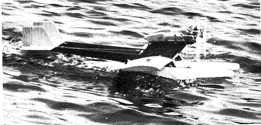
Sealander II in a fast taxi. Note how sponsons cause water to break aft of the props; a must for good seaplane design. Water in props robs power and can actually break or chip them!
