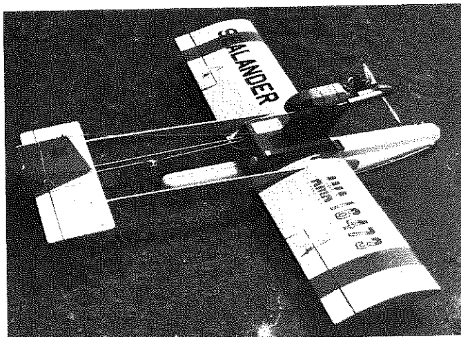
No radio gear in the floats, it's all in the center section and pod. Control linkage in the open and not tricky.
