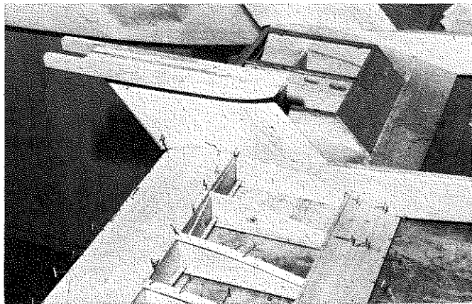
Sealander II center section during construction. Note aileron control tubing in place. Wing is semi-symmetrical but built on flat surface.
