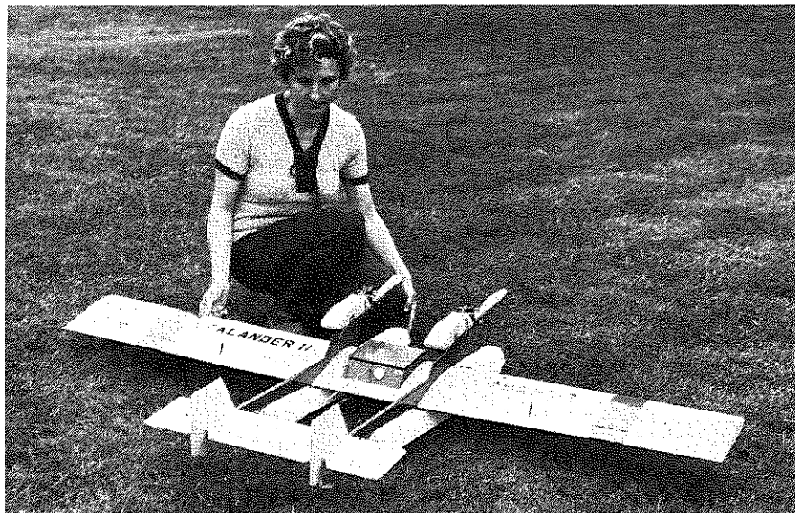
Sealand II and author's wife, Eleanor. Stretched wings, explained in text, are clearly visible. Original flights with 54 inch span, then 74, but 68 inch span is recommended. Again, see text.
