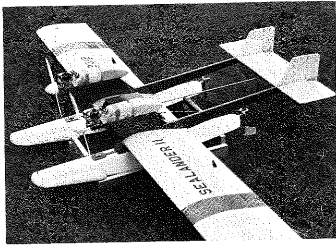
Both Sealanders have sponsons added to the floats. Lowers waterline and also deflects water spray away from props.
