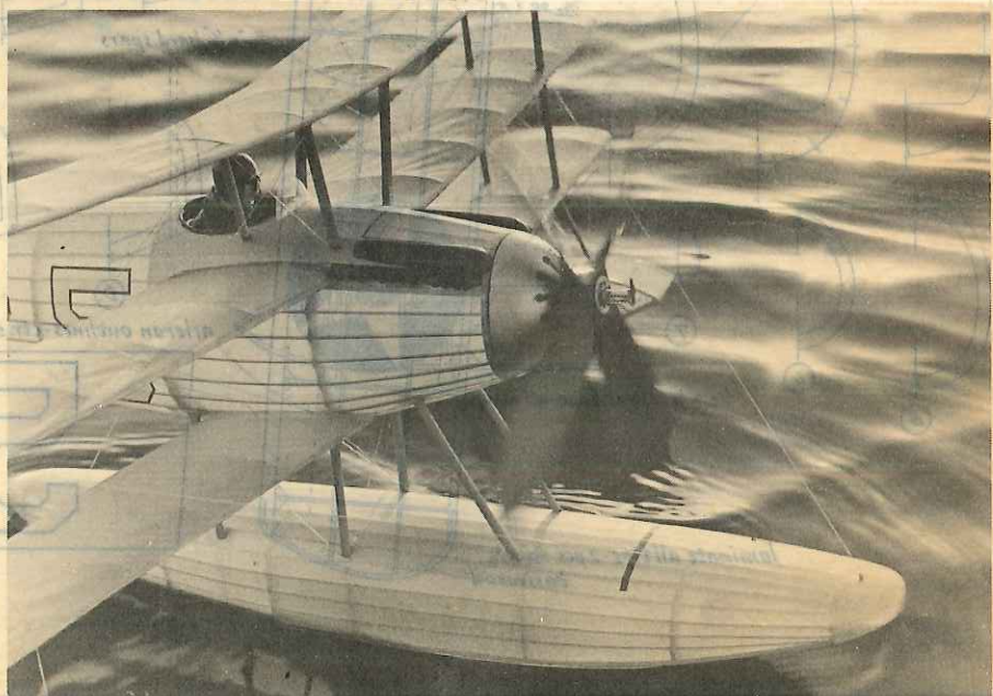
Bill used a freewheeling device on the prop for longer flights. Some of the struts are made from cocktail straws. Monofilament "wires" add greatly to the model's strength.
