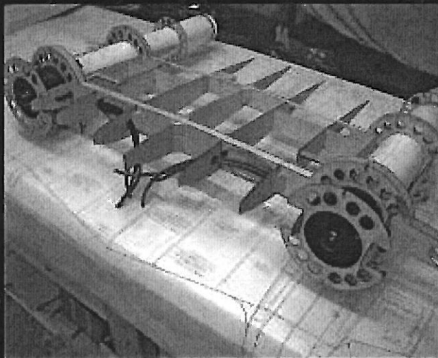
Below: The fan units were relocated from the front of the spar to behind it to allow for easier service and keyed into the wing ribs for support. The three motor wires are routed through the main spar. Jigs support the wing and keep it flat during construction.
