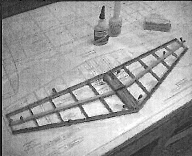
Left: The stabilizer is traditional built-up construction and features a symmetrical airfoil. The center ribs create a pocket for the internal elevator linkage.
