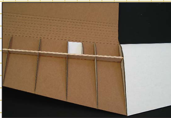
The right-wing-panel upper surface has been folded down and glued to the spar, ribs, and TE. Then the left wing is built in a similar fashion.
