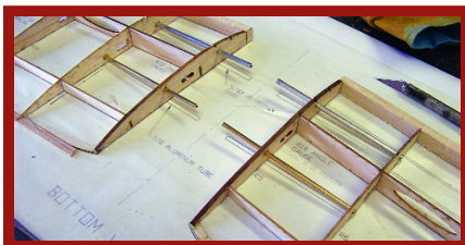
The 5/32-inch-OD and 1/8-inch-OD rear aluminum wing-attachment tubes are glued in place on the bottom wing assemblies.
