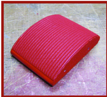
The top-wing center-section is covered with corrugated foam from Titanic Airlines, sanded to shape, and painted with Model Master Acryl.
