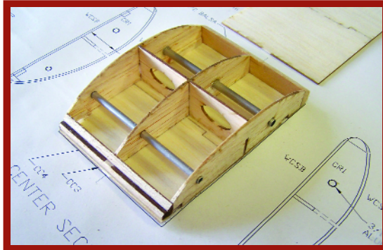
The top-wing center-section is built directly over its bottom sheeting, with plug-in wing-receiver tubes glued in place before the top skin is glued in place.
