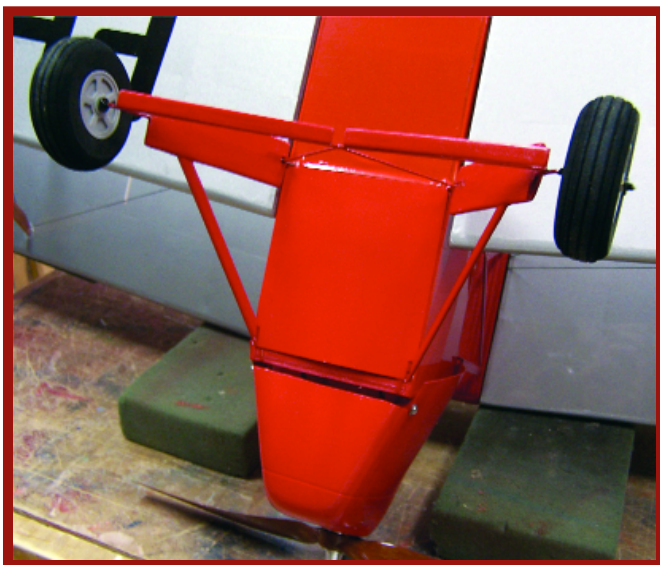
Battery access is through a plastic hatch on the fuselage bottom. Motor cooling air exits the gap at the bottom of the cowl at the firewall.
