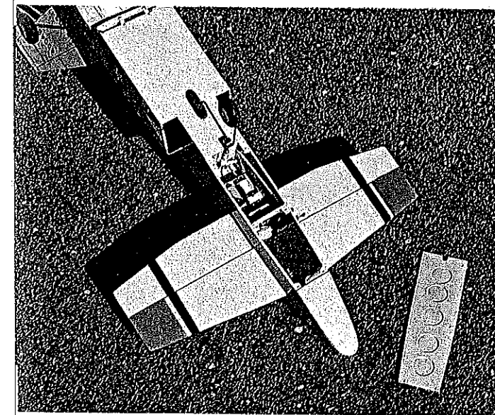
Left: Removable plywood hatch provides access to the radio gear. Battery fits into hollowed-out nose block. Throttle, rudder, and elevator servos are mounted far forward to help with balance. Right: A 24-in. aileron extension cable goes from the receiver back to the wing opening, where the servo is plugged in. Despite the forward radio installation, additional weight is necessary in the nose for balancing.
