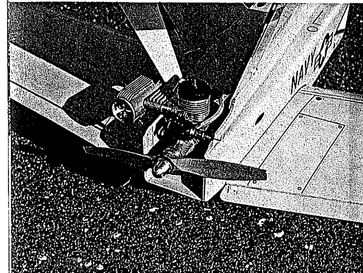
Left: Power comes from an HB .40 PDP Blitz engine and Zinger pusher prop. Read the author's comments in the text about props for pushers. A special muffler is available from HB that is ideal for a pusher installation. Right: Conventional strip aileron linkage couldn't be used inside the fuselage due to the engine location, so the servo was installed under a removable hatch with linkage direct to the ailerons. It works well.
