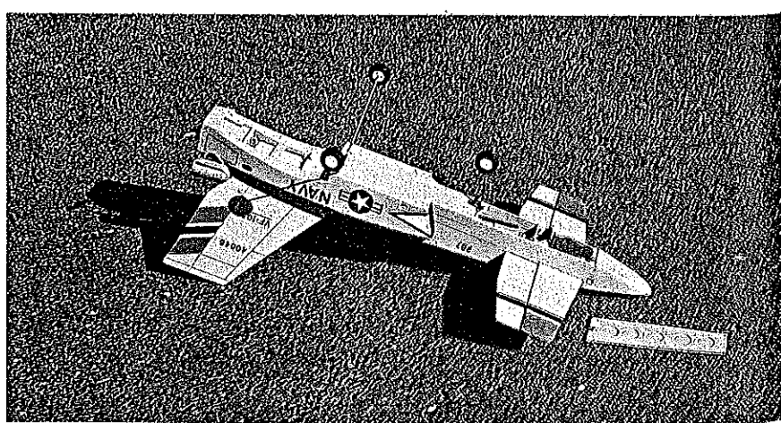
Left: Removable plywood hatch provides access to the radio gear. Battery fits into hollowed-out nose block. Throttle, rudder, and elevator servos are mounted far forward to help with balance. Right: A 24-in. aileron extension cable goes from the receiver back to the wing opening, where the servo is plugged in. Despite the forward radio installation, additional weight is necessary in the nose for balancing.
