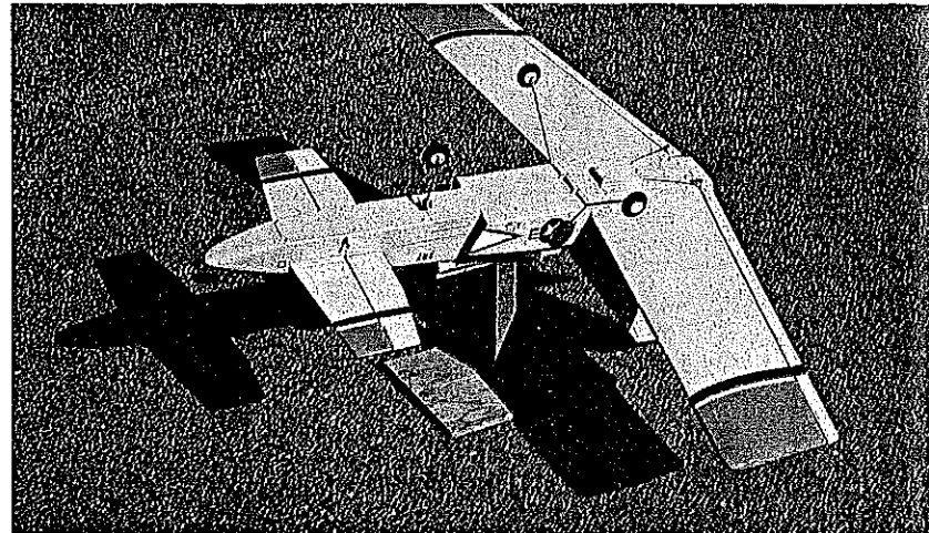
Left: Nick Nicholson, left, finished his Firebolt in an Air Force paint scheme based on the Grumman FSW aircraft now under construction. The author, right, chose a Navy scheme for his. Nick's model was the first Firebolt to fly; all the "bugs" were worked out on his model before the author's model was flown. Right: Two ¼-in. nylon bolts anchor the wing in place. The tricycle landing gear is mounted in the fuselage.
