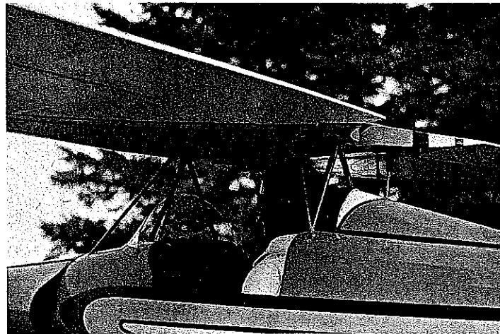
Steel wire cabane struts are anchored securely into fuselage, as they are the main load-carrying members. Note leather-covered headrest.
