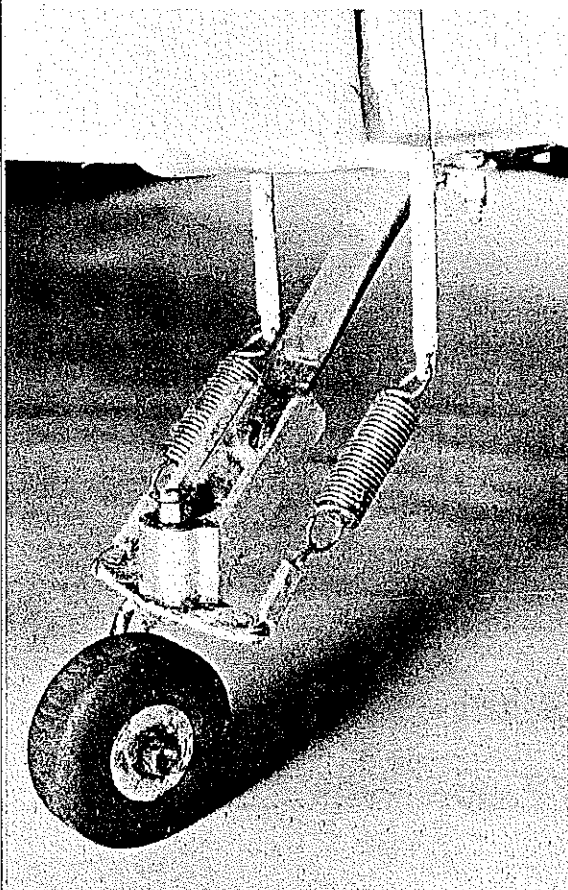
Flattened tread on the tail wheel is accomplished by holding coarse sandpaper against the tire while spinning it in a lathe or electric drill. Hardware store springs absorb ground shocks to avoid servo damage.
