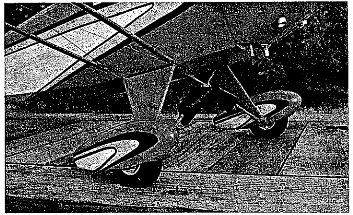
The full-size Pixie has fiberglass wheel pants. On the model they are balsa with a fiberglass cloth covering to help them withstand abuse.
