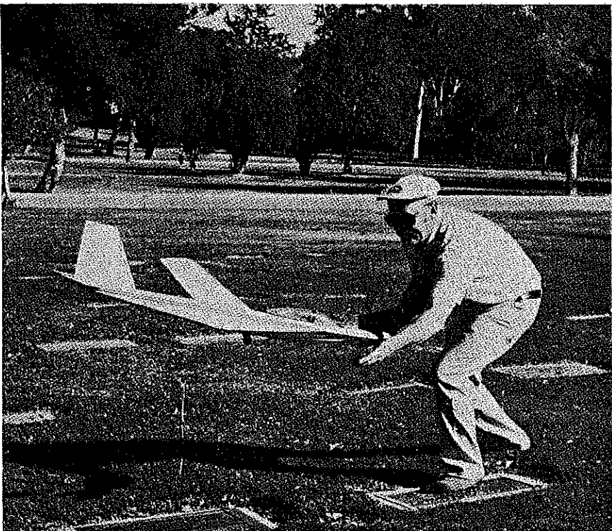
About to catch the Seville after a soaring flight is Bill Evans. Not only is this ship practical and simple, but it is enjoyably stable. The wing is foam cored, ply or balsa skin.
