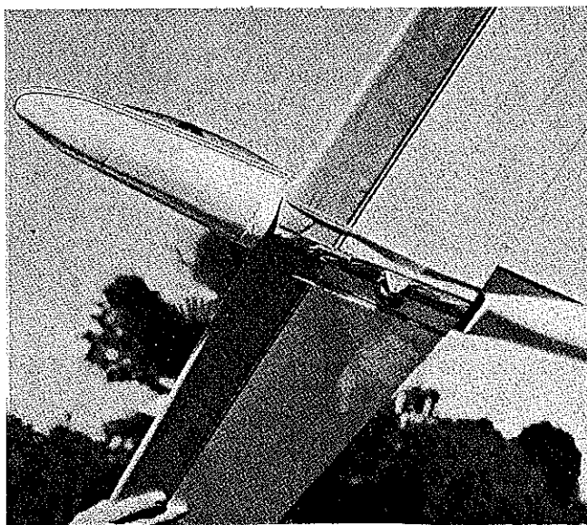
View from beneath showing the mono-wheel gear, tow hook and access hatch. The wheel does not interfere with the tow-line release.
